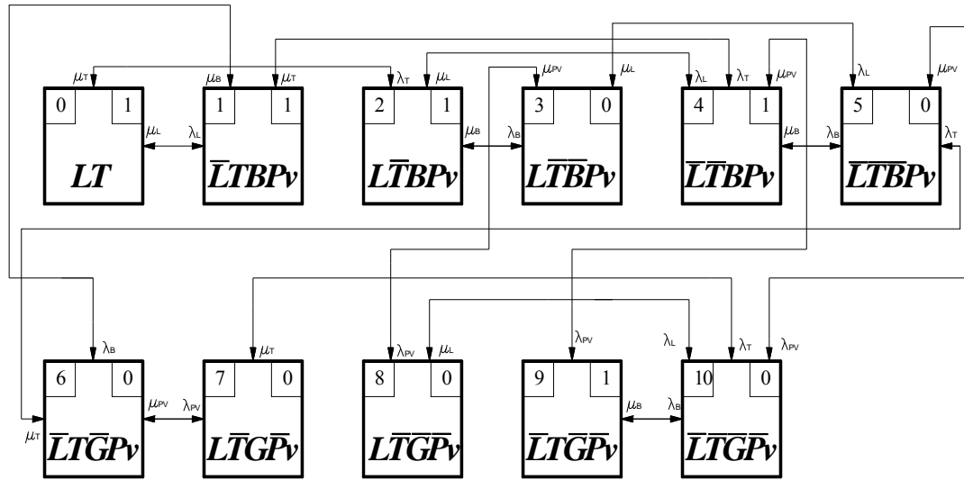
Figure 7.7. State Space Diagram for System with PV and Energy Storage System No Weather Conditions
